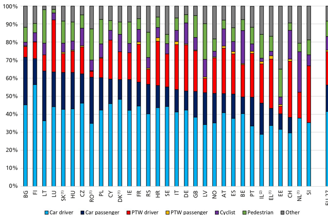
Figure 9. Proportion (%) of road deaths by road user group on rural roads ranked by the share of car driver and passenger road deaths taken together (2020- 2022 average). ( 1 )2019-2021, ( 2 )IL – data includes rural roads, motorways and off- road crashes. 11 EU average calculated for the period 2019-2021.
