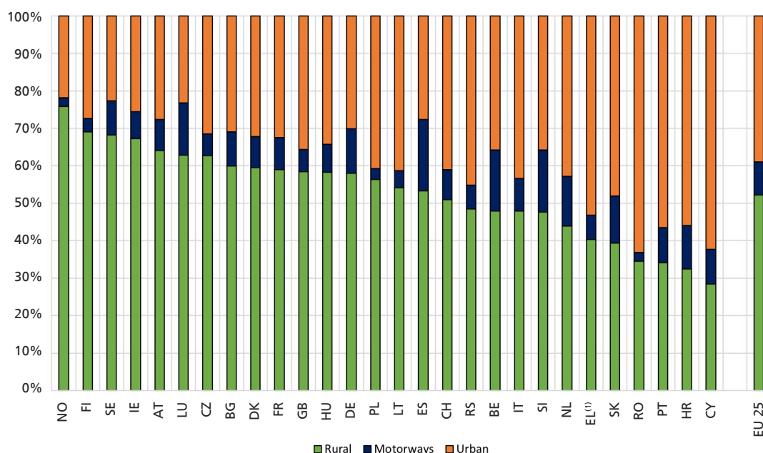
Figure 4. Proportion of road deaths per road type (2020-2022 average) in PIN countries ranked by the share of road deaths on rural roads. ( 1 )2019-2021. EU25: EU27 minus EE and MT due to lack of updated data.
